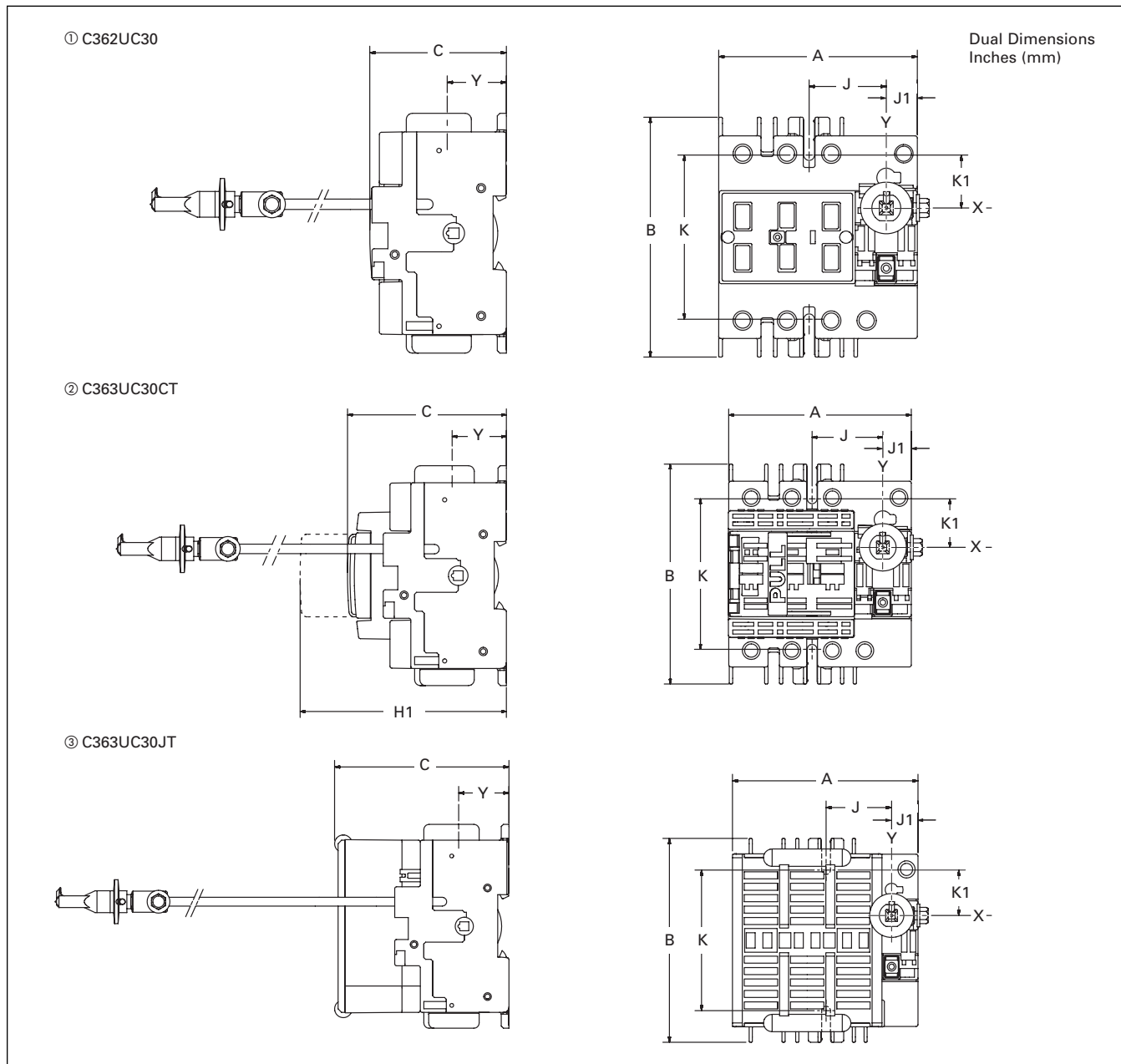
Figure 5. C-Frames
